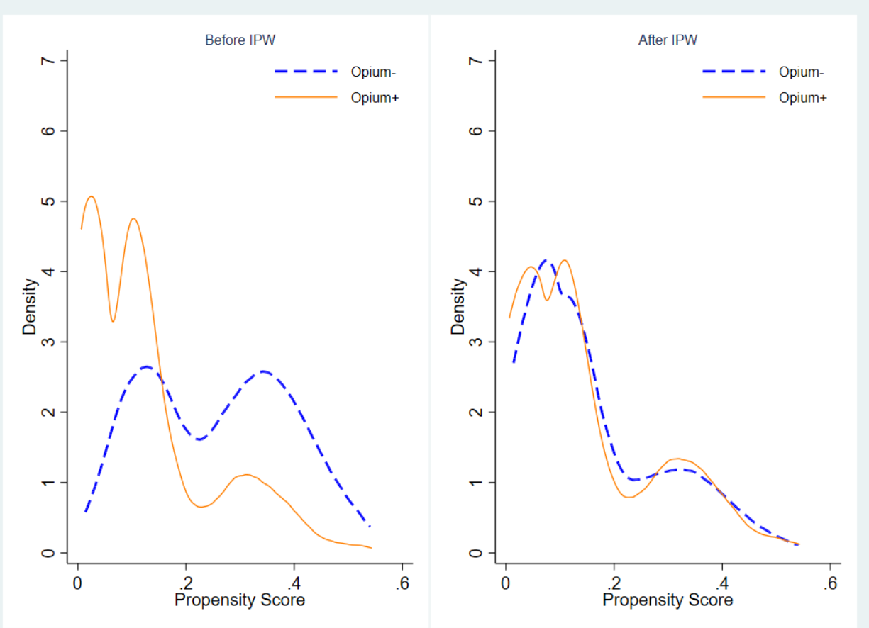
Supplementary Figure S1. Propensity score coverage before and after inverse propensity score weighting
